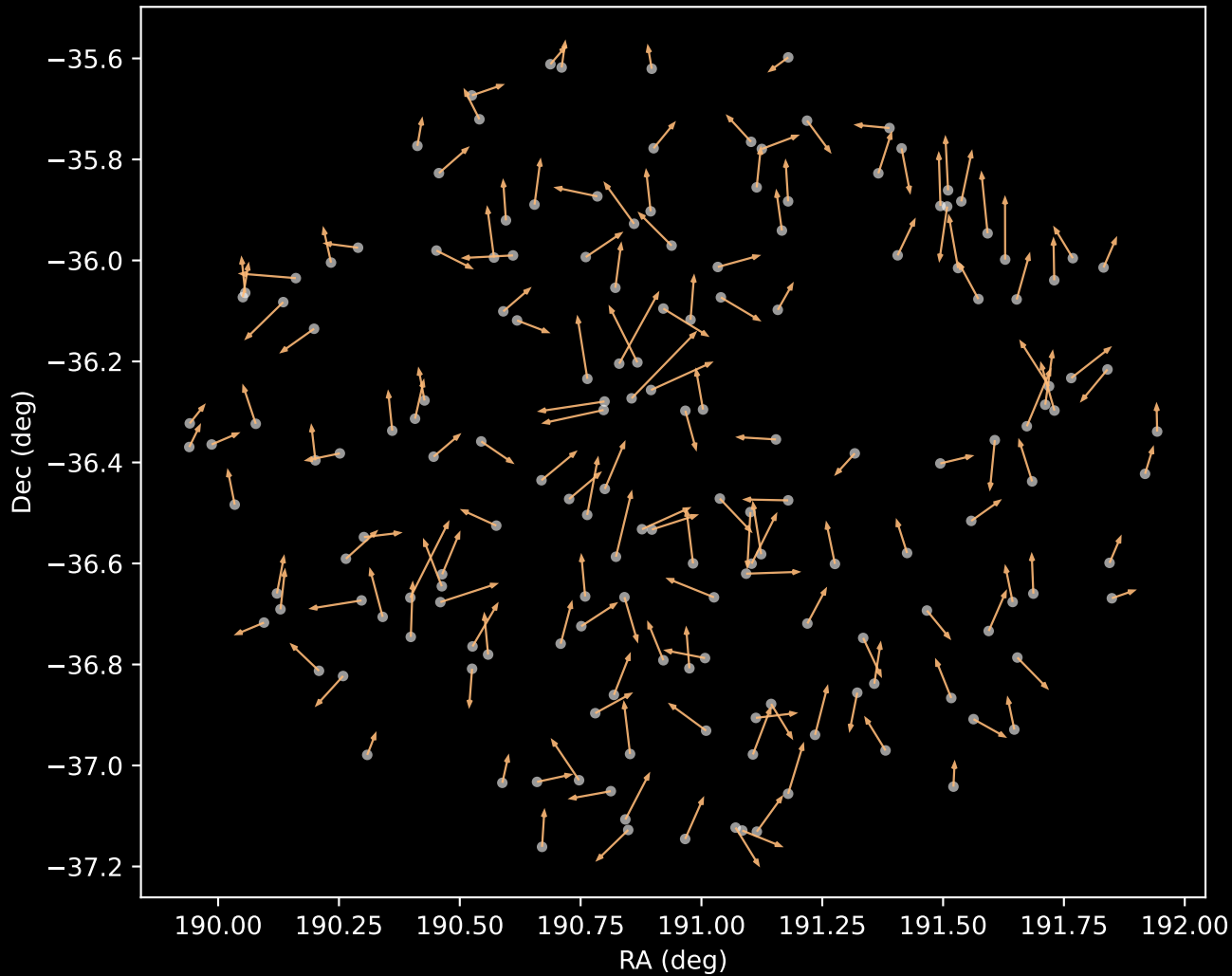
GALAH DR4 Cluster 3 Proper Motion Vectors (n=170)
