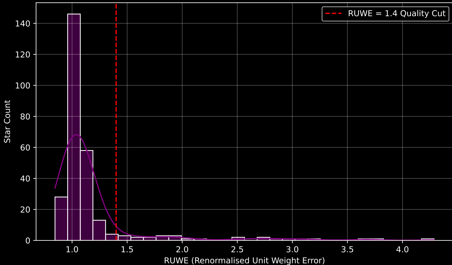
GALAH DR4 Field [1474] RUWE Distribution (n= 275)
