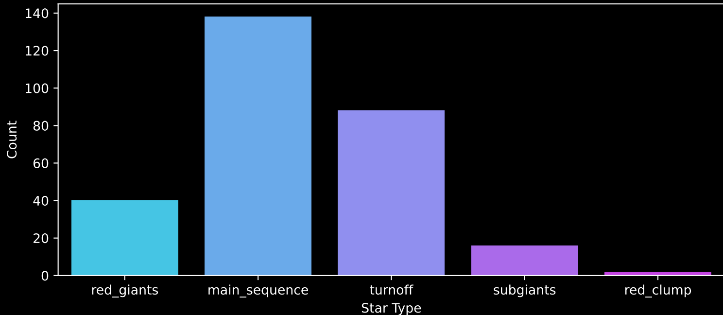
GALAH DR4 Field: [1474] Count plot of Star Type
